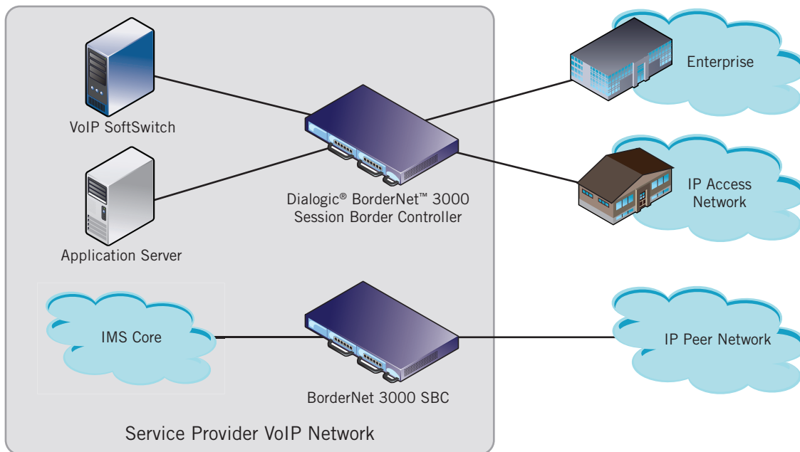
Figure 1. Dialogic® BorderNet™ 3000 Session Border Controllers in a Service Provider Network
